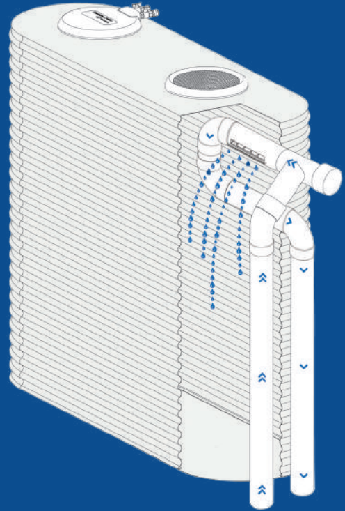
Filter is inside the tank, not exposed to sunlight therefore eliminating algae build up.
